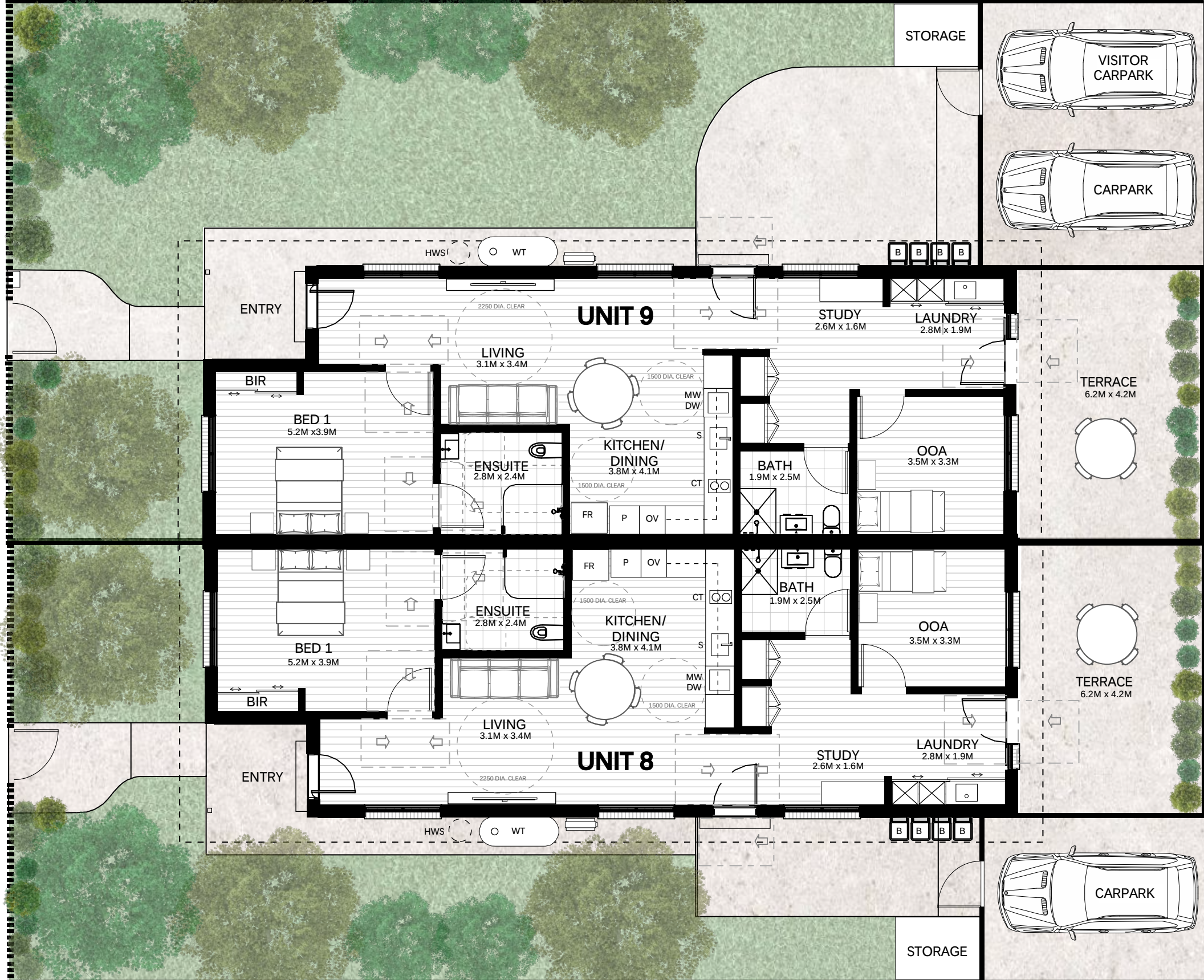
KEY PLAN
